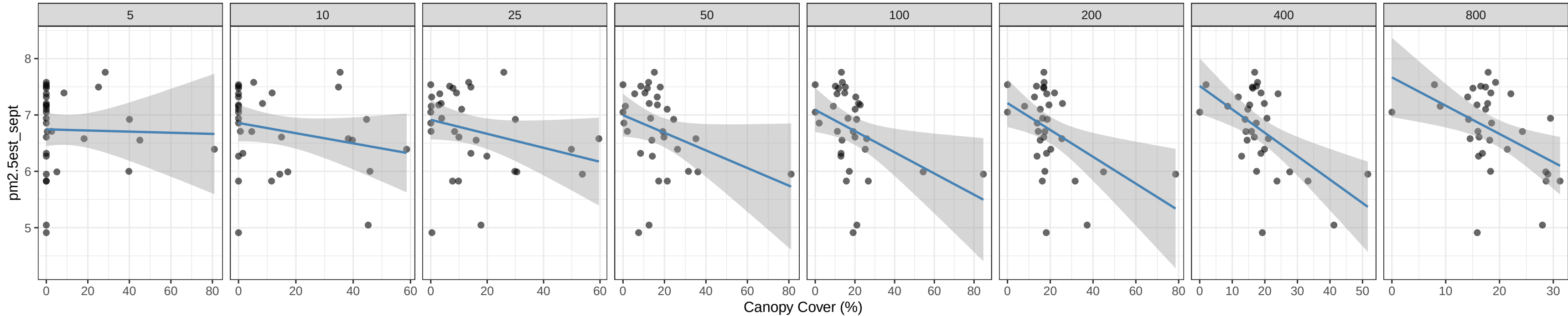
pm2.5est_sept vs Canopy Cover (%) by buffer radius
